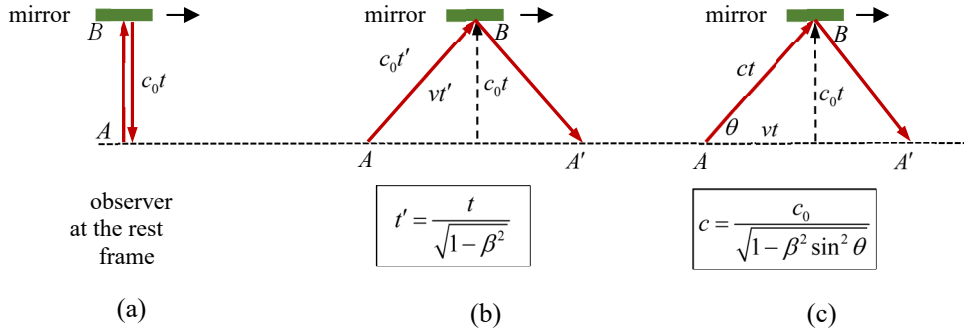
Fig. 5. Einstein's Gedanken experiment. (a) Light path in the rest frame. (b) In the laboratory frame. Explained with time dilation. (c) In the laboratory frame. Explained with anisotropic velocity.
