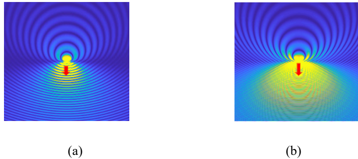
Fig.2. The field patterns of a moving Hertzian dipole. The red arrows show the moving directions. (a) \beta = 0.6 . (b) \beta = 0.8 .
