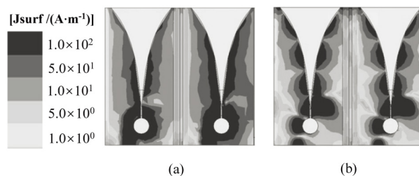
图4 天线的表面电流分布. (a) f = 2 \text{ GHz} , d = 0.13 \lambda . (b) f = 15 \text{ GHz} , d = 1.03 \lambda .
