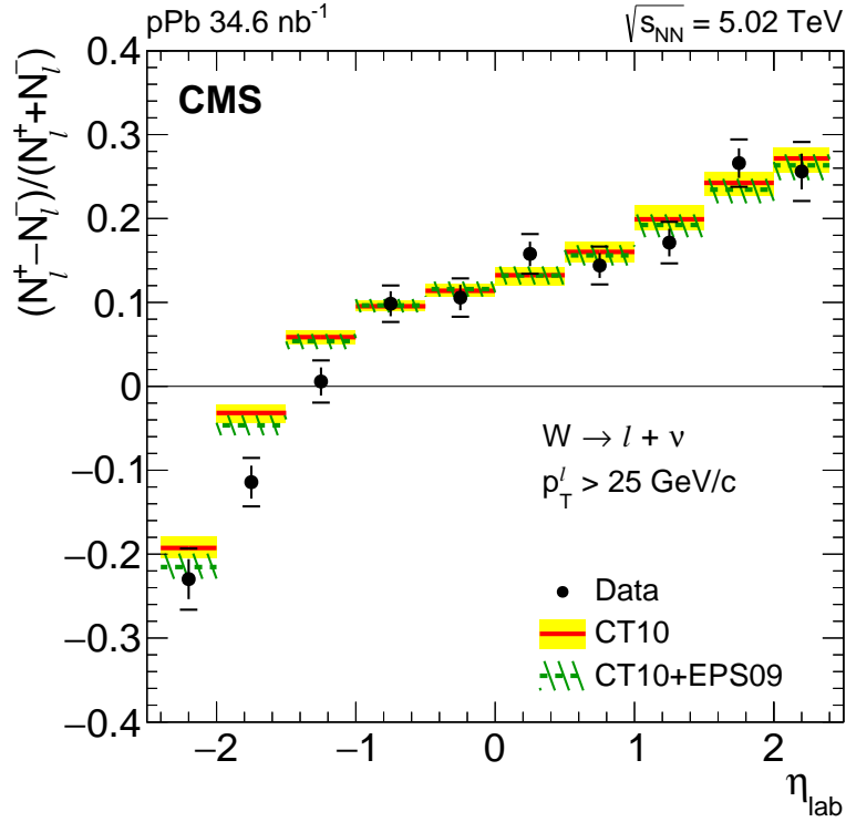
Figure 4: Lepton charge asymmetry, (N_\ell^+ - N_\ell^-)/(N_\ell^+ + N_\ell^-) , as a function of the lepton pseudorapidity. Error bars represent the statistical uncertainties, while brackets show statistical and systematic uncertainties summed in quadrature. Theoretical predictions with (CT10+EPS09, dashed green line) and without (CT10, solid red line) PDF nuclear modifications are also shown, with their uncertainty bands.
