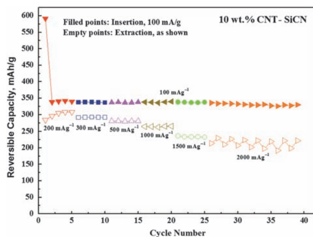
Figure 5. Change in capacity with increasing current densities in CNT-SiCN composite anode. In these tests the insertion current density was held constant at 100 mA g -1 , while the extraction current density was varied as shown in the figure.
