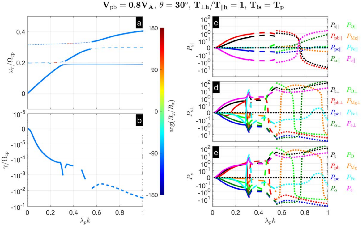
Figure 6. The Alfvén wave mode in the corona when there are no instabilities. (a) The real frequency and (b) damping rate of the Alfvén wave mode; (c) the parallel, (d) perpendicular and (e) total energy transfer rate of particles and wave mode. The solid, dashed and dotted lines in (c)–(e) represent different regions of wave mode shown in (a). The horizontal axis \lambda_p k represents normalized wavevector, where \lambda_p is the proton inertial length.
